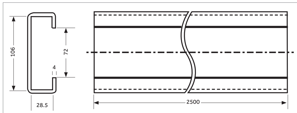
42357-2.4MTR & 42357-3.0MTR PROFILE
